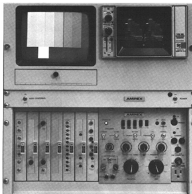
CCU and monitoring for the BC-230B version
